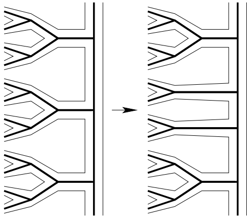
FIGURE 1. Increasing number of vertices along \partial_0 X
