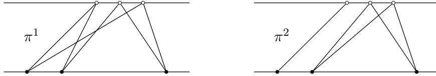
Figure 5: The optimal transports from Example 10.1
