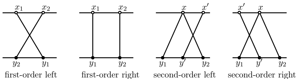
Figure 3: Forbidden configurations in the monotonicity properties
