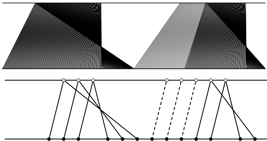
Figure 2: Simulations of the Decreasing Supermartingale Transport. We observe an interval of Right-Curtain kernels on the left, followed by an interval of Hoeffding–Fréchet kernels and another interval of Right-Curtain kernels. The destinations of these intervals preserve the original order.
