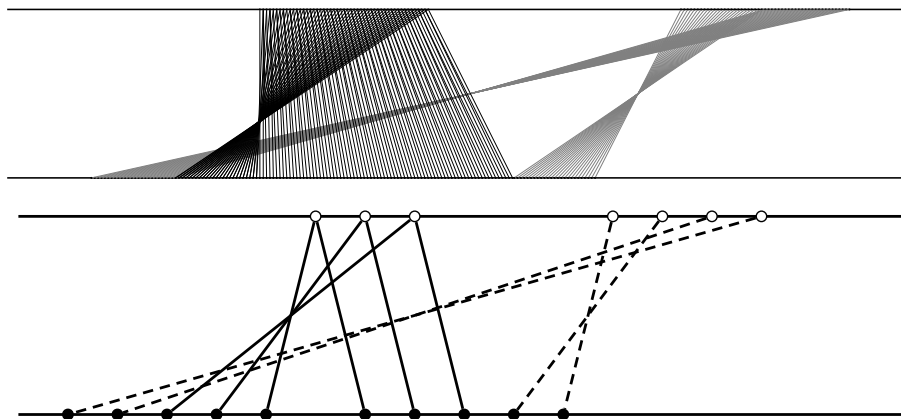
Figure 1: Simulations of the Increasing Supermartingale Transport. We observe an interval of Left-Curtain kernels (black/continuous) on the left and an interval of Antitone kernels (gray/dashed) on the right. The destinations of the right interval are on both sides of the destinations of the left one.
