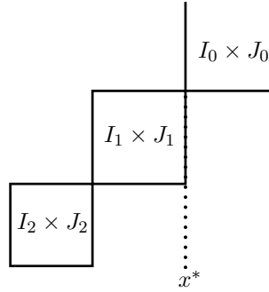
Figure 4: Illustration of two martingale components, separated from the supermartingale component I_0 \times J_0 by the maximal barrier x^* .
