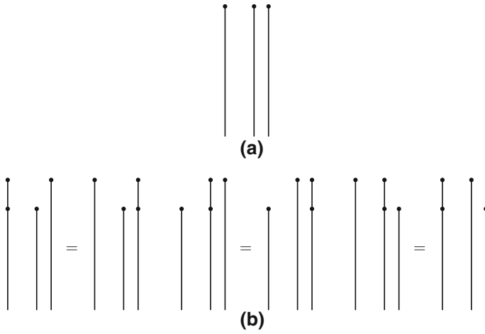
Fig. 7 a An element in \mathcal{R}_1^0(3) and b three pairs of equivalent cut diagrams in \mathcal{R}_1(3) associated with this element
