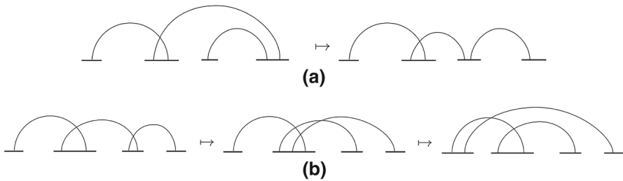
Fig. 5 Moving a pair of intersecting arcs, one of which has the leftmost end, to the left, for the case where the first arc end met belongs to the right interval: a the second end of the arc met also belongs to the right interval; b the arc met intersects the second one
