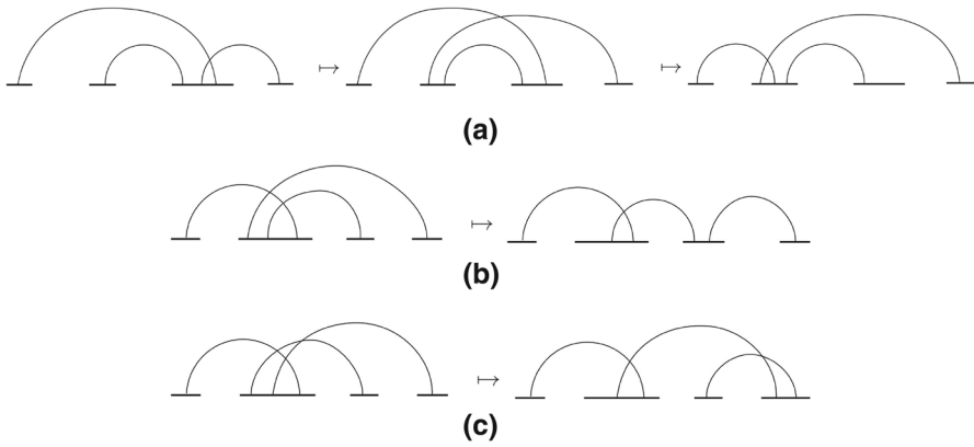
Fig. 4 Moving a pair of intersecting arcs, one of which has the leftmost end, to the left, for the case where the first arc end met belongs to the left interval: a the second end of the arc met also belongs to the left interval; b the second end of the arc met does not belong to the left interval, and the arc does not intersect the second one; c the second end of the arc met does not belong to the left interval, and the arc intersects the second one
