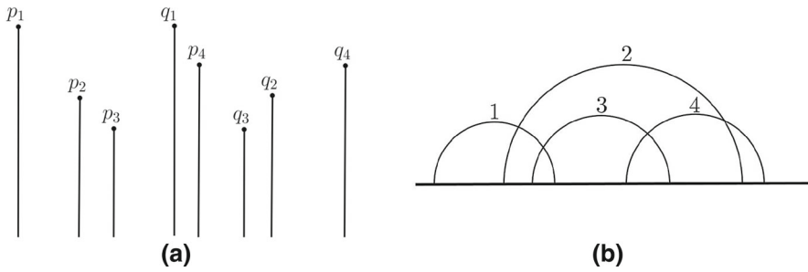
Fig. 1 a A cut diagram and b the corresponding arc diagram
