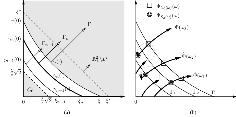
FIG 3. (a) The stopping regions (each arrow at the boundary of a region points toward the interior of that region), and (b) three sample paths and the optimal stopping times S_2 and U_0 for the optimal stopping problems V_2 in (5.1) and V in (4.12), respectively.
