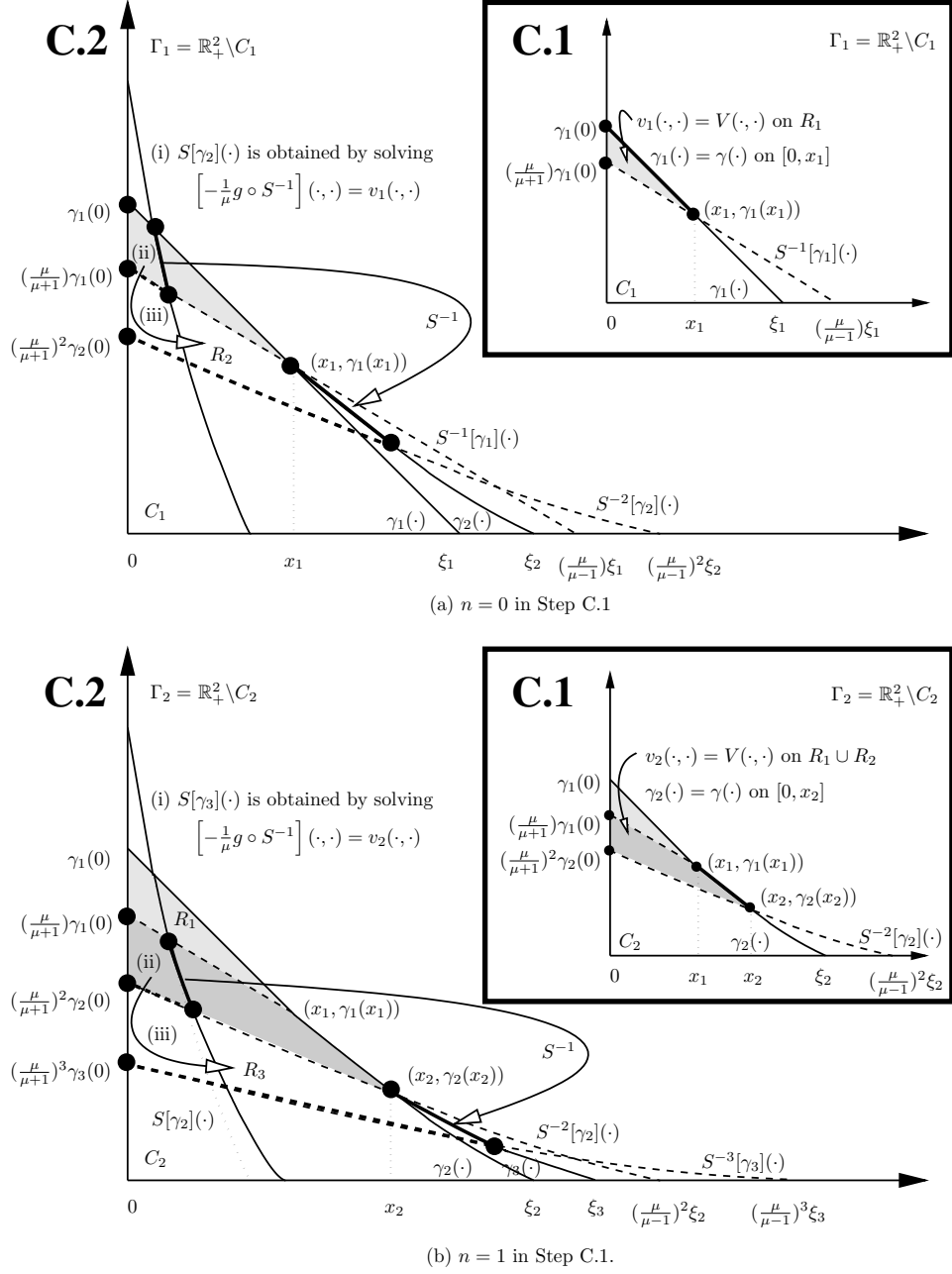
FIG 4. Case I: \lambda is “large.” The illustration of Method C, see page 33: Steps C.1 and C.2 when (a) n = 0 , and for (b) n = 1 in Step C.1.
