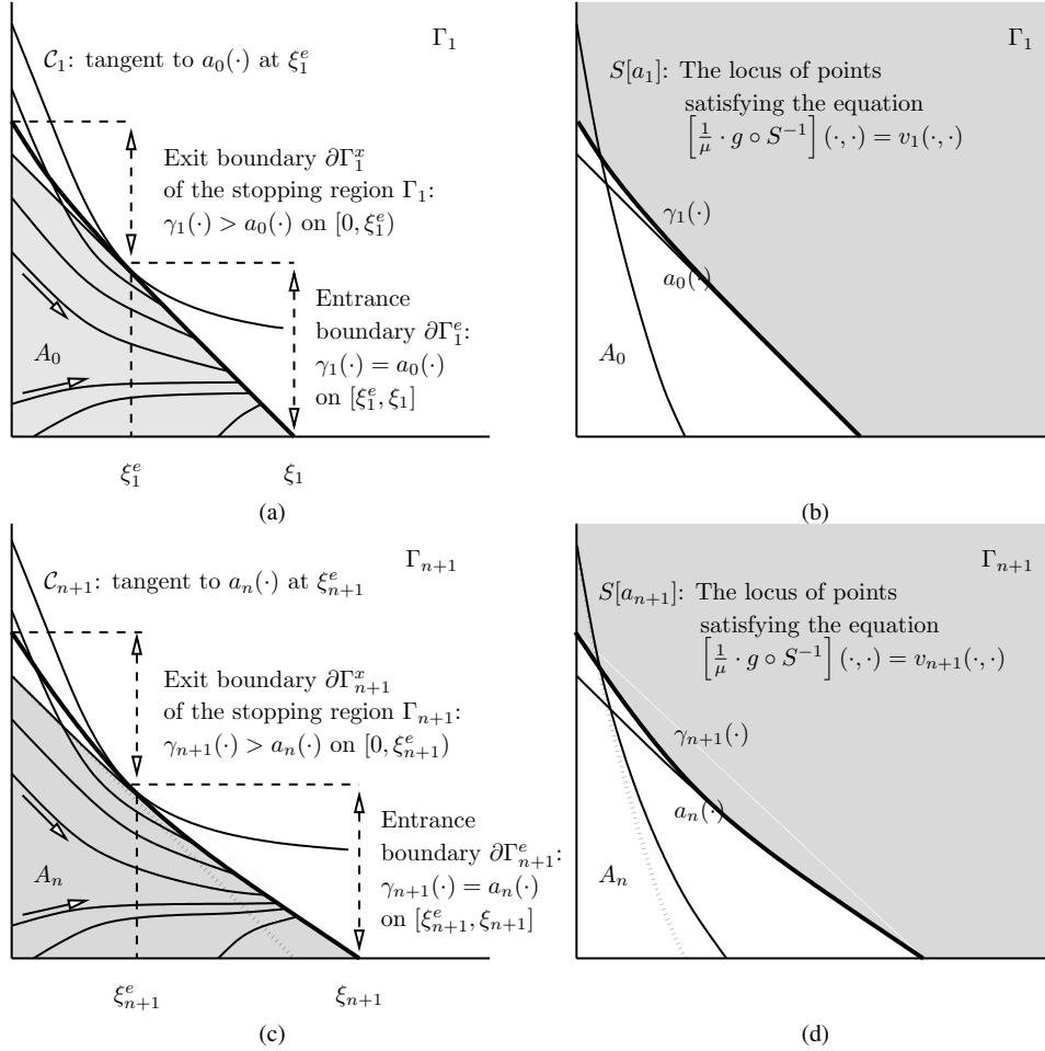
FIG 5. Figures (a) and (b) illustrate Steps D.1 and D.2 of Method D page 42 for n = 0 , and Figures (c) and (d) for a general n .
