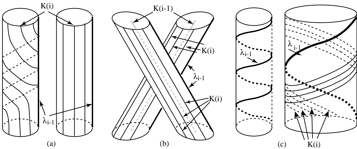
Figure 13: Iterated torus knots.
