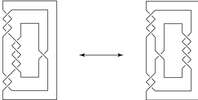
Figure 16: The simplest example which illustrates our conjecture
