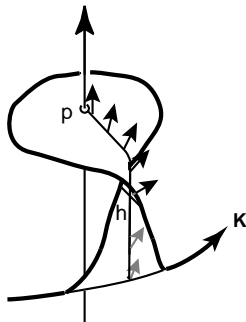
Figure 4: A positive elliptic singularity ( p ) and a positive hyperbolic singularity ( h ).
