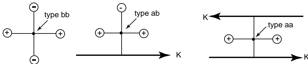
Figure 5: The three types of hyperbolic singularities.
