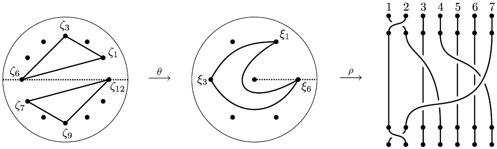
Fig. 12. Translating pairs of symmetric polygonal braids in B_{2n-2}^B to Artin generators in B_n^A .
