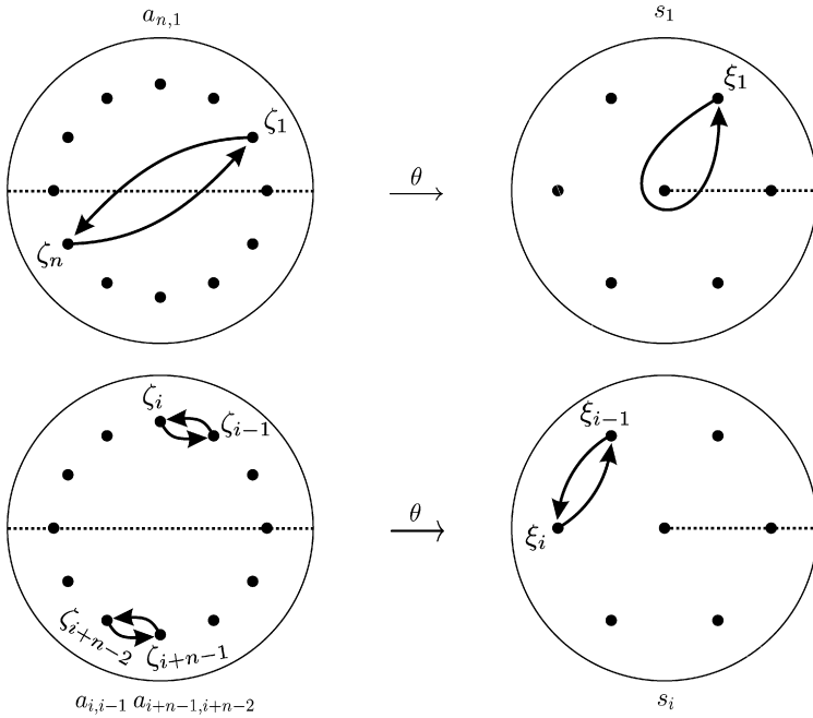
Fig. 9. The map \theta transforms the symmetric braids on the left-hand side to the generators of \mathcal{A}(\mathbf{B}_{n-1}) on the right-hand side.
