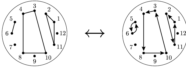
Fig. 7. A simple element of B_{12}^B , which is a product of three polygonal braids. It is the braid (a_{11,2}a_{2,1})(a_{10,8}a_{8,4}a_{4,3})(a_{6,5}) , where the three factors (the polygonal braids) commute.
