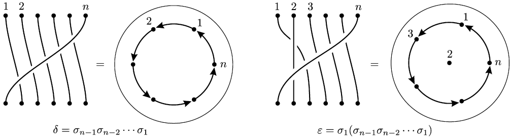
Fig. 1. The periodic elements \delta and \varepsilon .
