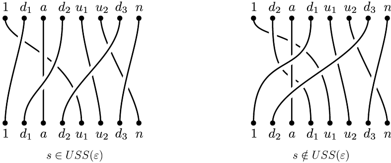
Fig. 4. Two simple braids in B_8^A whose permutations are cycles of length 7. By Proposition 13, the first one is conjugate to \varepsilon and the second one is not. As in Fig. 2, the exponent sums of the two braids differ; the exponent sum of second one is 12, while the exponent sum of conjugates of \varepsilon \in B_8^A is 8.
