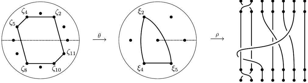
Fig. 13. Translating a single symmetric polygonal braid in B_{2n-2}^B to Artin generators in B_n^A .
