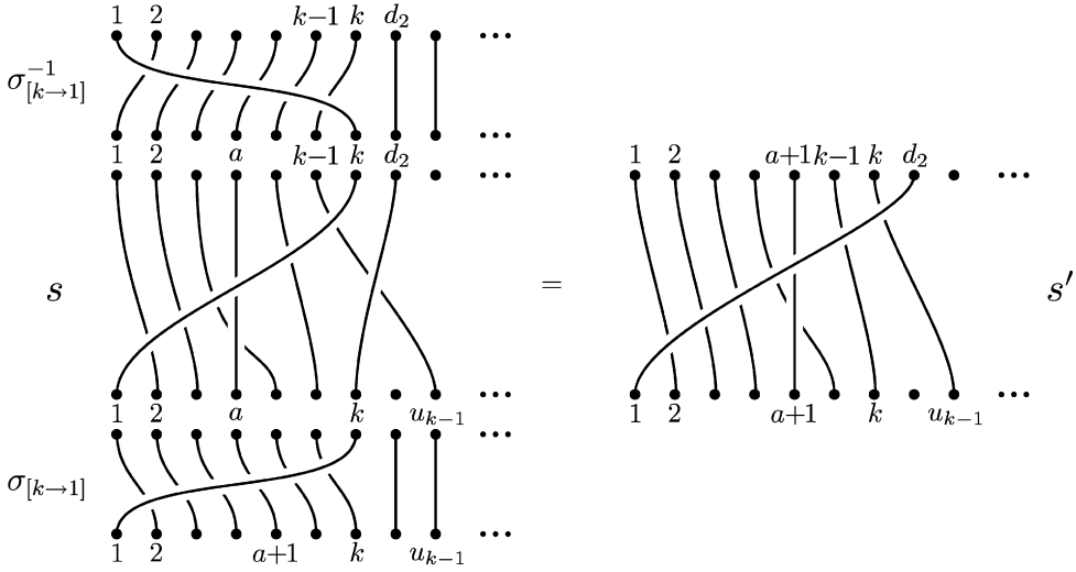
Fig. 5. Conjugating s to s' when a < k .
