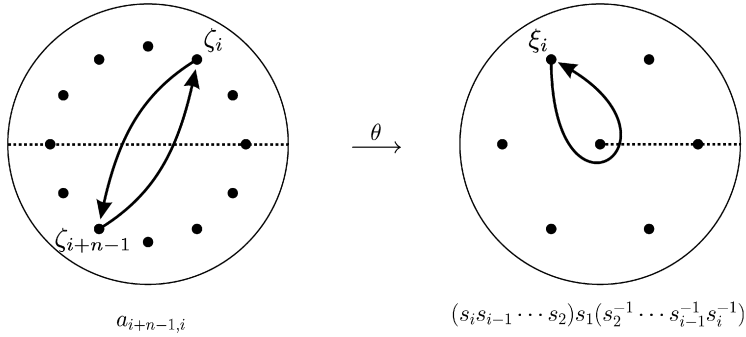
Fig. 10. The image under \theta of a_{i+n-1,i} .
