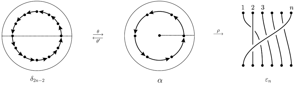
Fig. 11. A geometric interpretation of \rho(\theta(\delta)) = \varepsilon .
