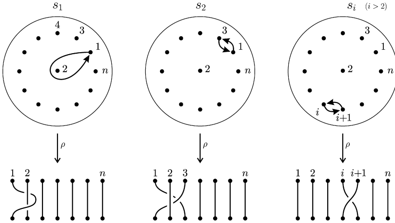
Fig. 8. The generators of \mathcal{A}(\mathbf{B}_{n-1}) , represented as braids on \mathbb{D}^2 \setminus \{0\} , and their images under the isomorphism \rho: \mathcal{A}(\mathbf{B}_{n-1}) \rightarrow P_{n,2} .
