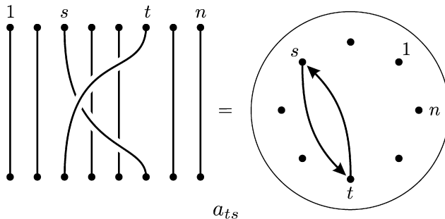
Fig. 6. The band generator a_{ts} .
