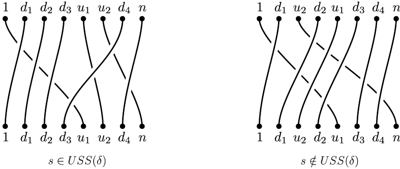
Fig. 2. Two simple braids in B_8^A whose permutations are cycles of length 8. By Proposition 10, the first one is conjugate to \delta and the second one is not. Notice that the exponent sum of the second one (i.e., the number of crossings or the letter length, in this case) is 9, while the exponent sum of conjugates of \delta \in B_8^A is 7.
