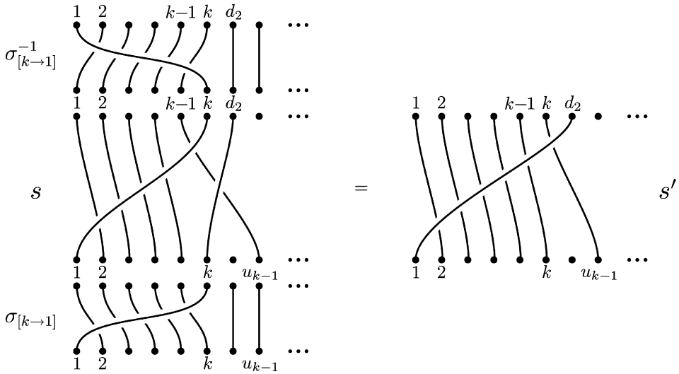
Fig. 3. Conjugating s to s' .
